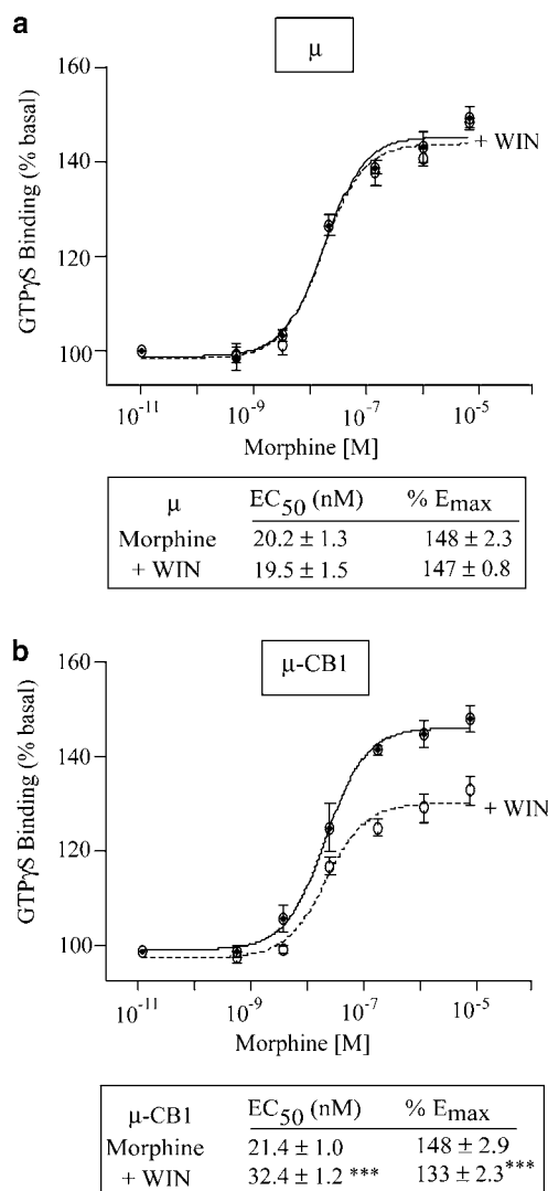
Figure 2 Signaling in cells expressing \mu or \mu -CB1 receptors. HEK-293 cells expressing \mu receptors alone (a) or coexpressing \mu and CB1 receptors (b) were permeabilized and subjected to a [ 35 S]-GTP \gamma S binding assay (see Methods) with the indicated (0–10 -5 M) concentrations of morphine in the absence or presence of 10 nM WIN 55,212-2. The EC 50 and E max changes were determined by GraphPad Prism and are indicated in the box below each graph. The data represent mean ± s.e.m. ( n = 12). Statistically significant differences were determined by the Student's t -test. *** P < 0.001 ( n = 12).
