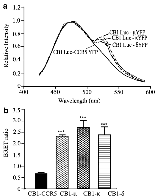
Figure 1 Opioid and CB1 cannabinoid receptor interactions in live cells. (a) Light emission was monitored from HEK-293 cells cotransfected with 1 µg of CB1-Luc and either 1 µg of µ-YFP (dashed line), κ-YFP (dotted line), δ-YFP (hatched line) or 1 µg of CCR5-YFP (solid line). The BRET assay was carried out as described in Methods. The peak of light emission by luciferase is seen at 470 nm and the peak resulting from the BRET between CB1-Luc and opiate-YFP-tagged receptors is seen at 530 nm. A representative sample of an experiment is shown. (b) The light intensities were expressed as a BRET ratio (ratio of the intensity of light emitted at 530 nm versus the intensity of light emitted at 470 nm) for each experimental paradigm compared to cells expressing only CB1-Luc. Statistically significant differences were determined by one-way ANOVA. *** P < 0.001 ( n = 15–18; F = 9.731; R squared = 0.3989).
